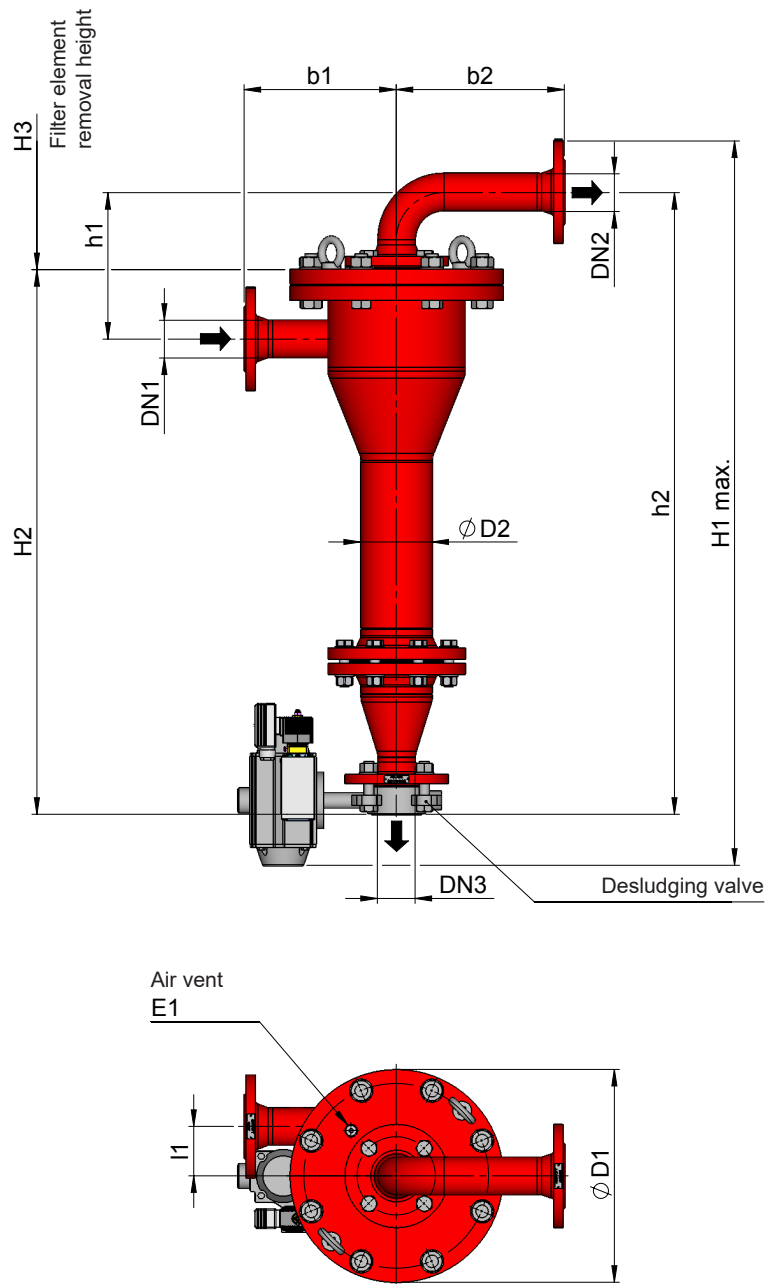
Size AutoFilt® ATF-2, ATF-2.5 to ATF-3 (Drawing shows carbon steel variant)
