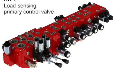
LX-6 + HX-1 Primary control valve combination solution
