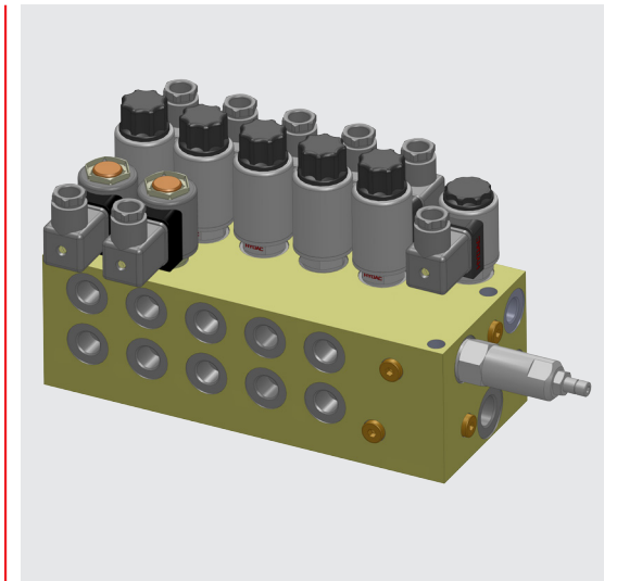
Compact control block with cartridge valves
