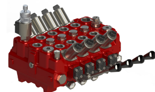
RS 220 Open centre primary control valve
