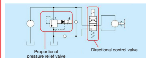
Example of fan control application
