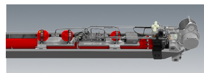
Telescoping cylinder (11 m) with semi-integrated hydraulic control
